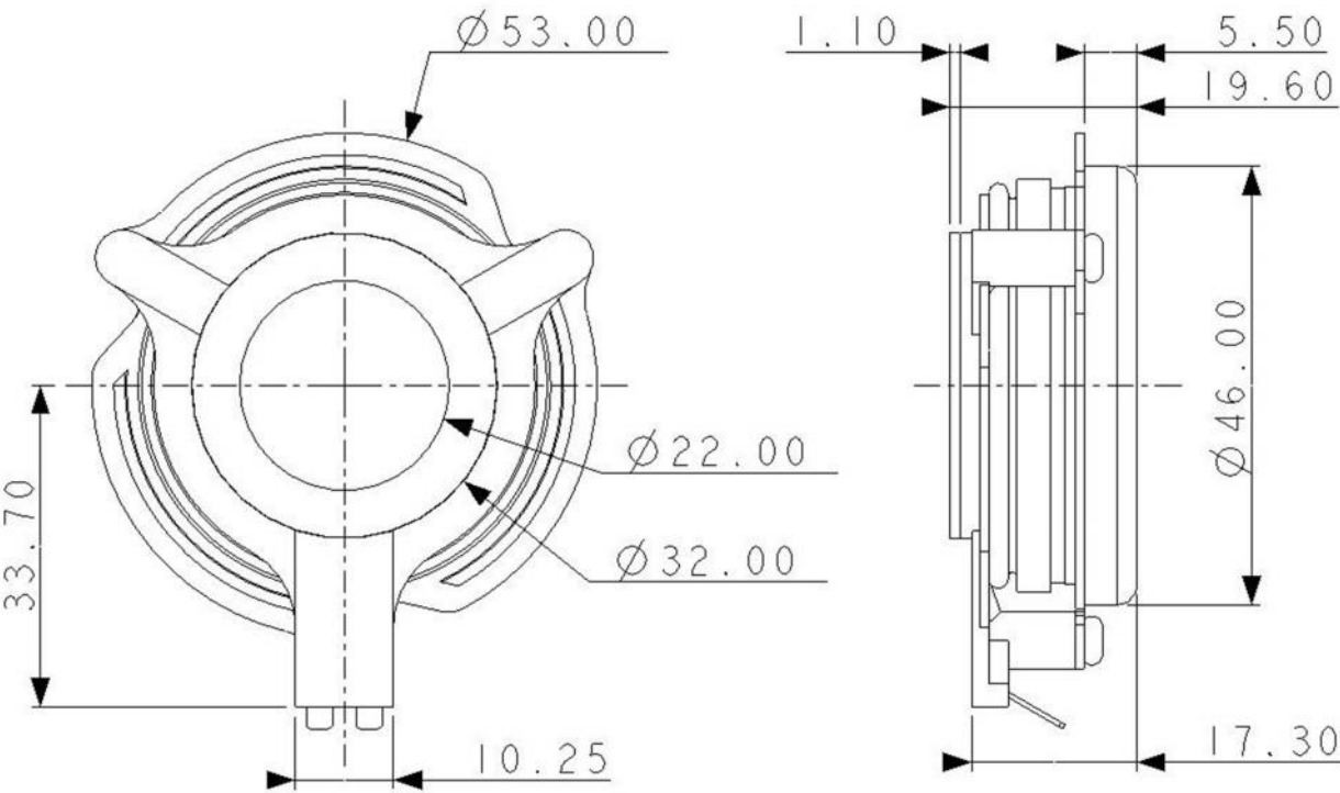
Figure 2. Nominal dimensions
